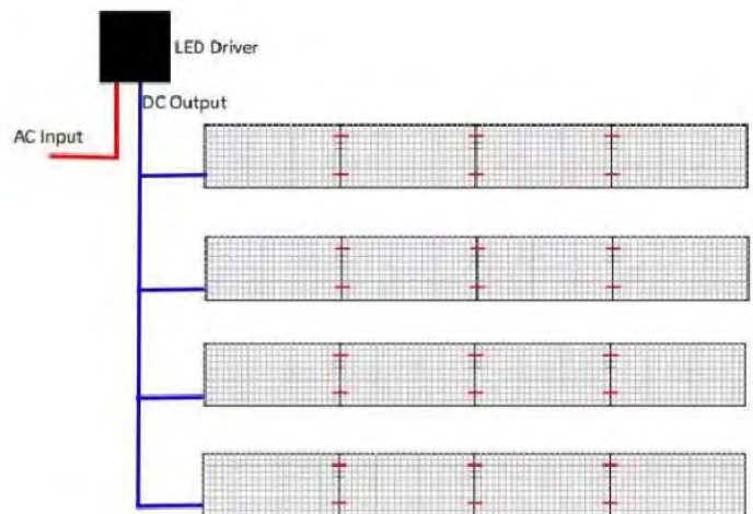
2. Connection method two/连接方式2
